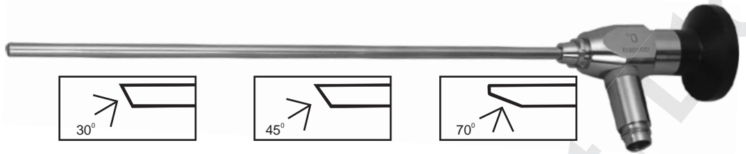
S.002 Sinuscope 4mm 30°, wide angle, Working length 175mm
